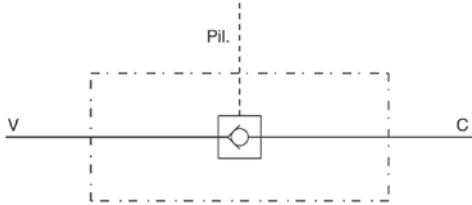
Single Pilot Operated Check Valves - 3 Way, In Line
