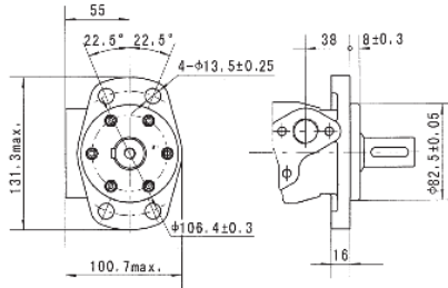
4 SAE A 4 Bolt Magneto Mount
