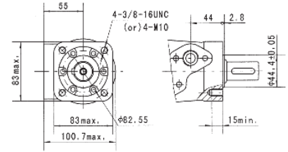
H5 4 Bolt Square Mount
