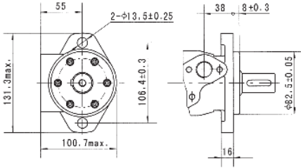
2 Standard SAE 2 Bolt Mount
