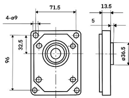
E2 Front Cover
