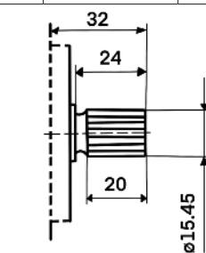
DP16/32-30° -9T
