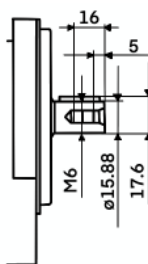
P12 5/8" Straight Keyed Shaft
