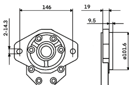
A8 SAE B Front Cover
