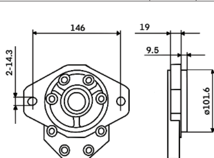
A8 SAE B Front Cover
