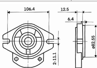
A2 SAE A Front Cover
