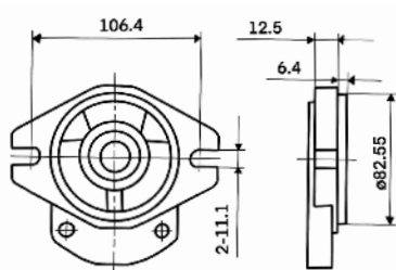
A2 SAE A Front Cover
