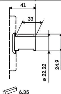
P16 7/8" Straight Keyed Shaft
