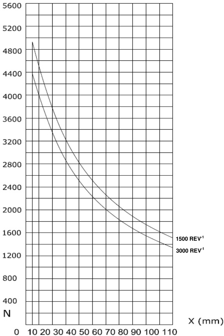
DIAGRAMMA A CARICHI RADIALI AMMISSIBILI GRAPHIC OF RADIAL LOAD
