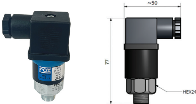
F4 Series Pressure Switch - Adjustable - M3 Type Connector
